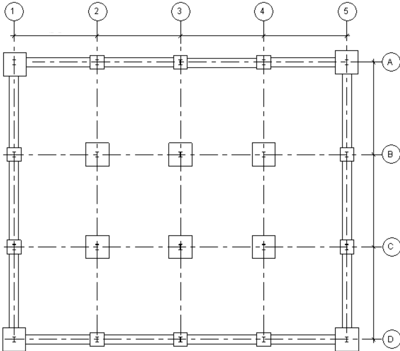
Retail Building: Foundation Plan
